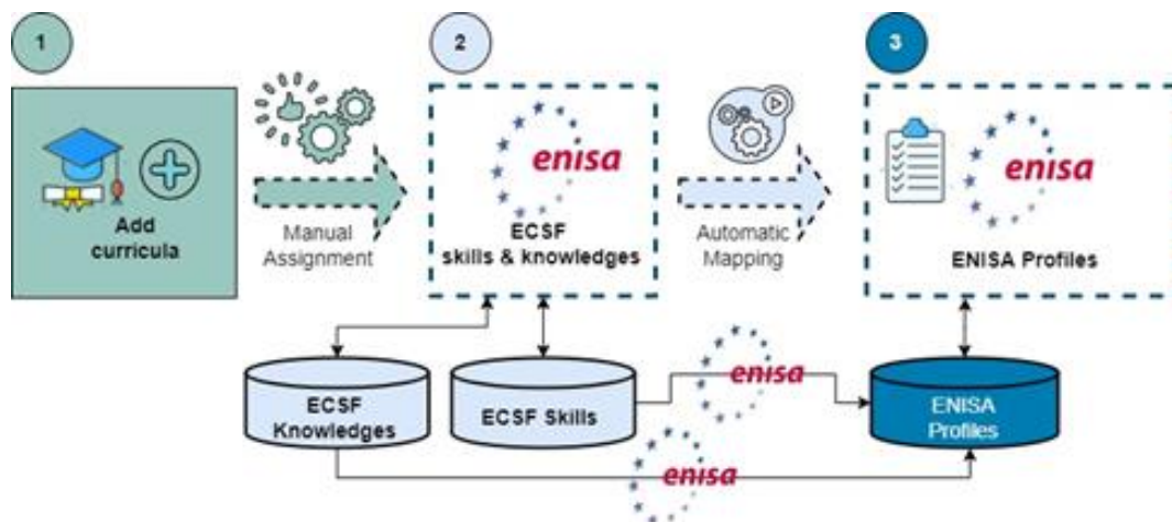
Figure 29 CCD-v2 app's back-end architecture and logic.
