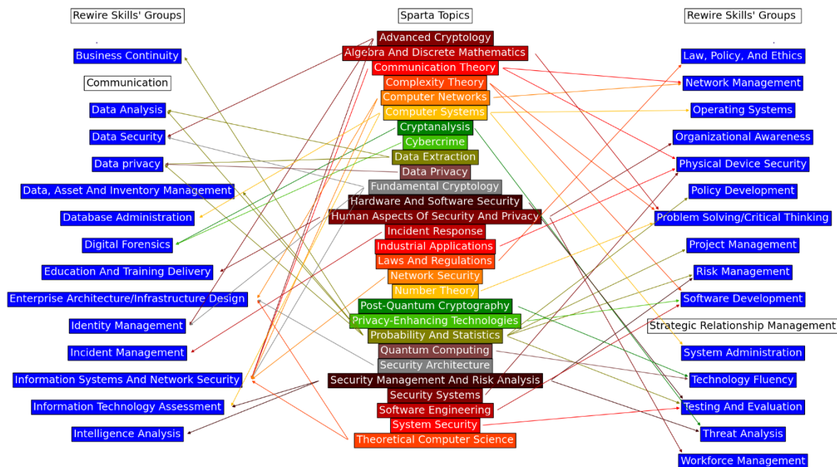
Figure 16 The mapping of SPARTA topics and REWIRE groups.
