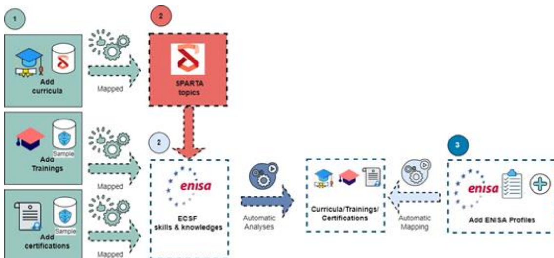
Figure 33 Cybersecurity Profiler (CSP) app's back-end architecture and logic (bilateral features).
