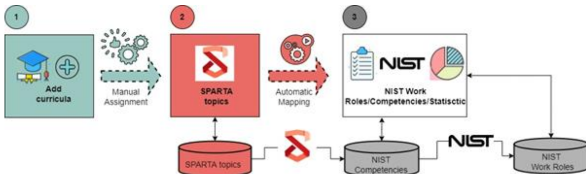
Figure 27 CCD-v1 app's back-end architecture and logic.
